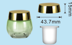
编号:E013 简称:赫莲娜30g盖+15g内胆 规格:43.7mmx15mm
