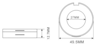
HG7224B SIZE:W49.5*H12.7MM
