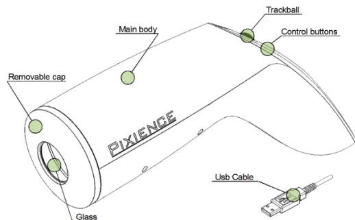
Figure 1 : C-Cube main components
