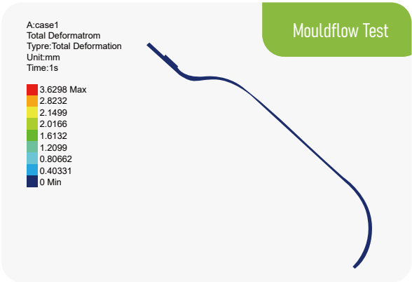
Mouldflow Test
